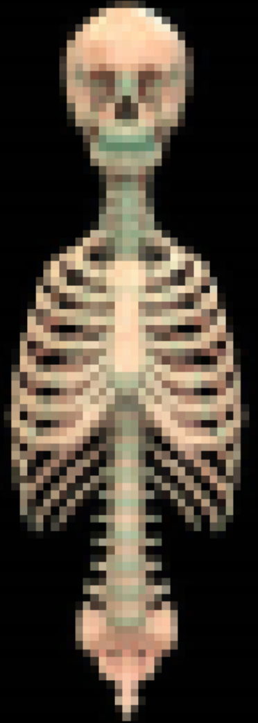
Axial Skeleton
